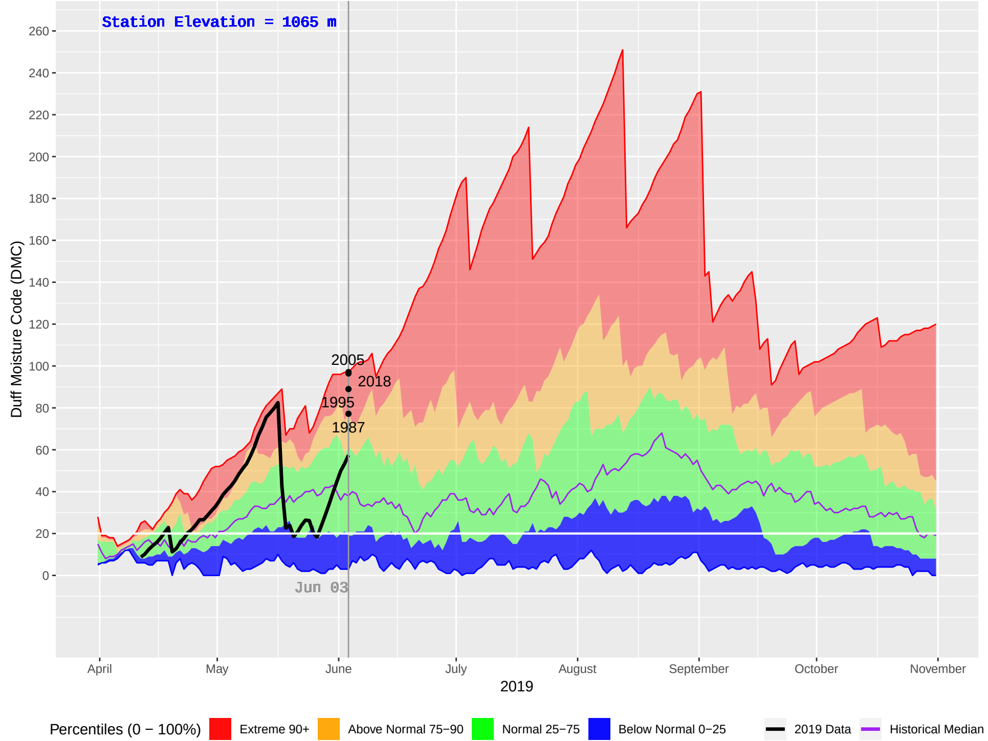
PLACE LAKE (212) : Historical (1981–2018), Current (2019) Daily Duff Moisture Code (DMC)
