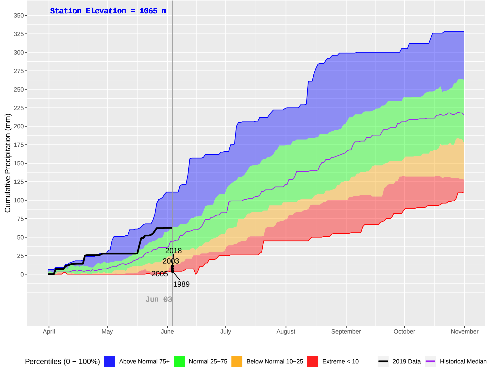
PLACE LAKE (212) : Historical (1981–2018), Current (2019) Daily Cumulative Precipitation
