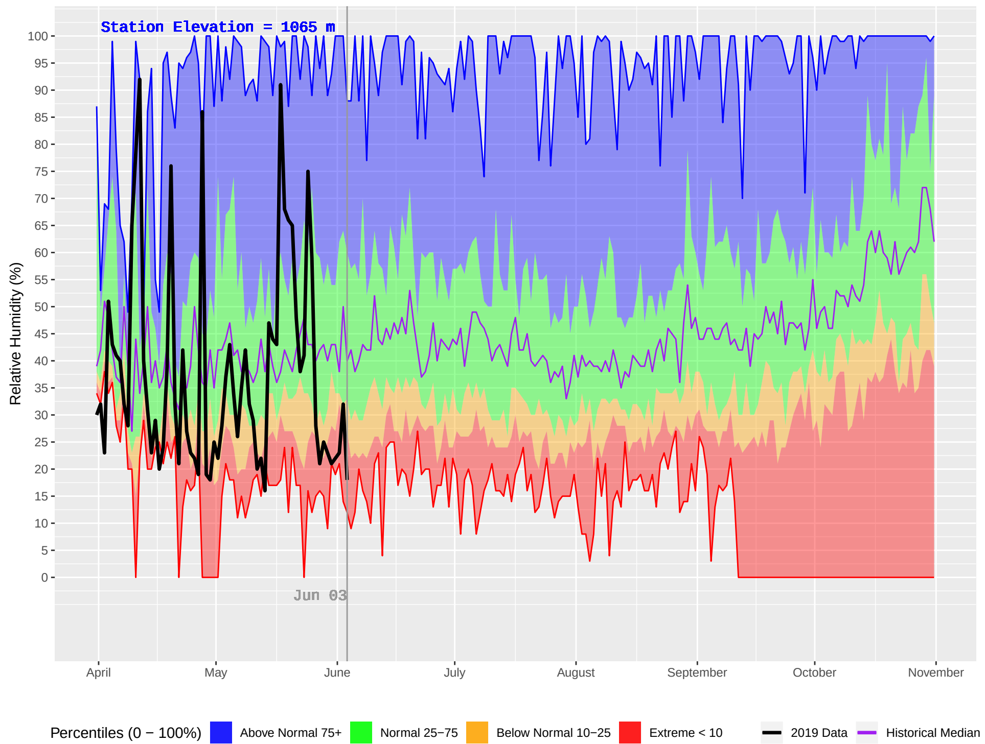
PLACE LAKE (212) : Historical (1981–2018) and Current (2019) Daily Relative Humidity
