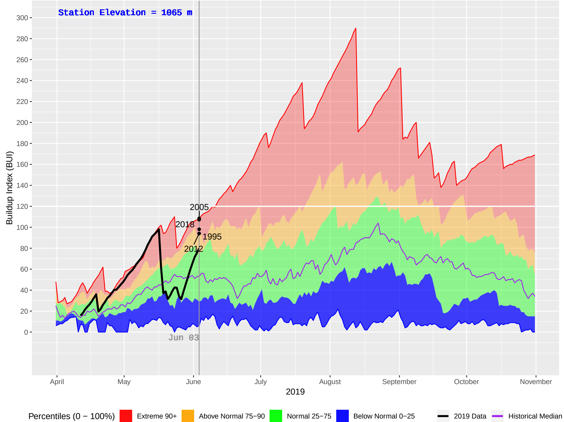
PLACE LAKE (212) : Historical (1981–2018), Current (2019) Daily Buildup Index (BUI)
