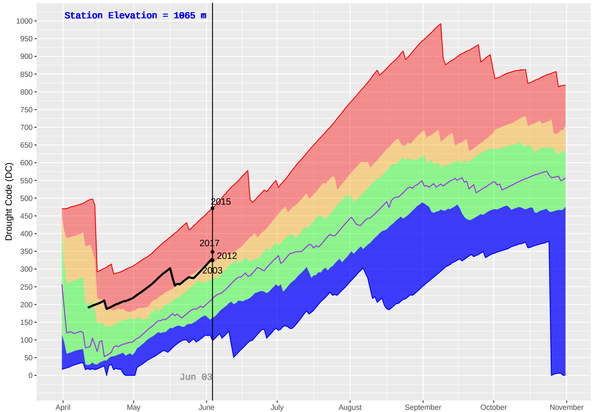
PLACE LAKE (212) : Historical (1981–2018) and Current (2019) Daily Drought Code (DC)
