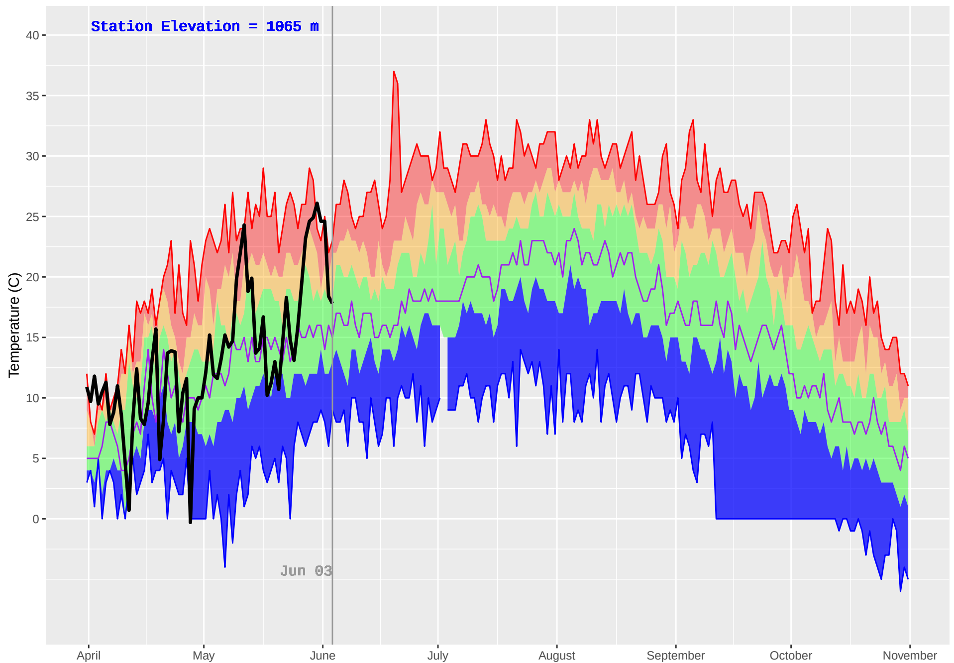
PLACE LAKE (212) : Historical (1981–2018) and Current (2019) Daily Temperature
