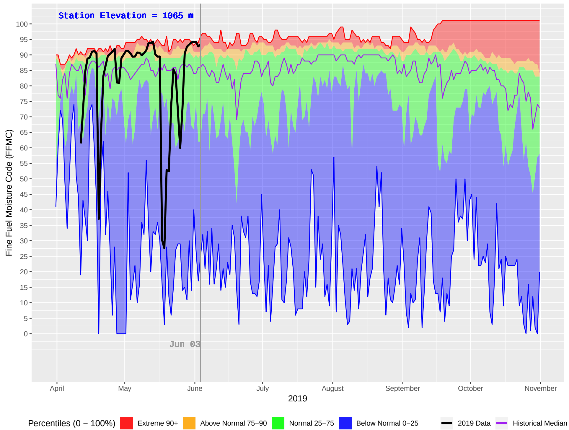
PLACE LAKE (212) : Historical (1981–2018) and Current (2019) Daily Fine Fuel Moisture Code (FFMC)
